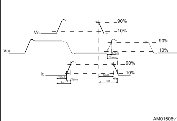
Figure 30. Switching waveform
